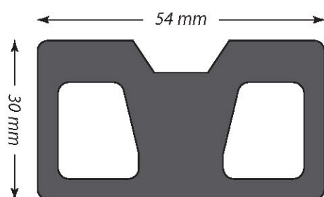
COMPOSITE JOIST
